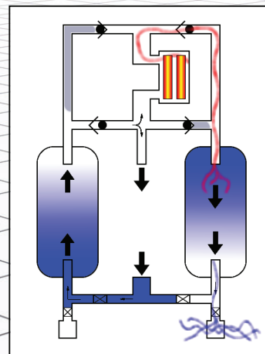
External Heat Conduction
