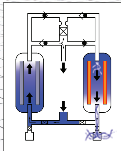
Internal Heat Conduction
